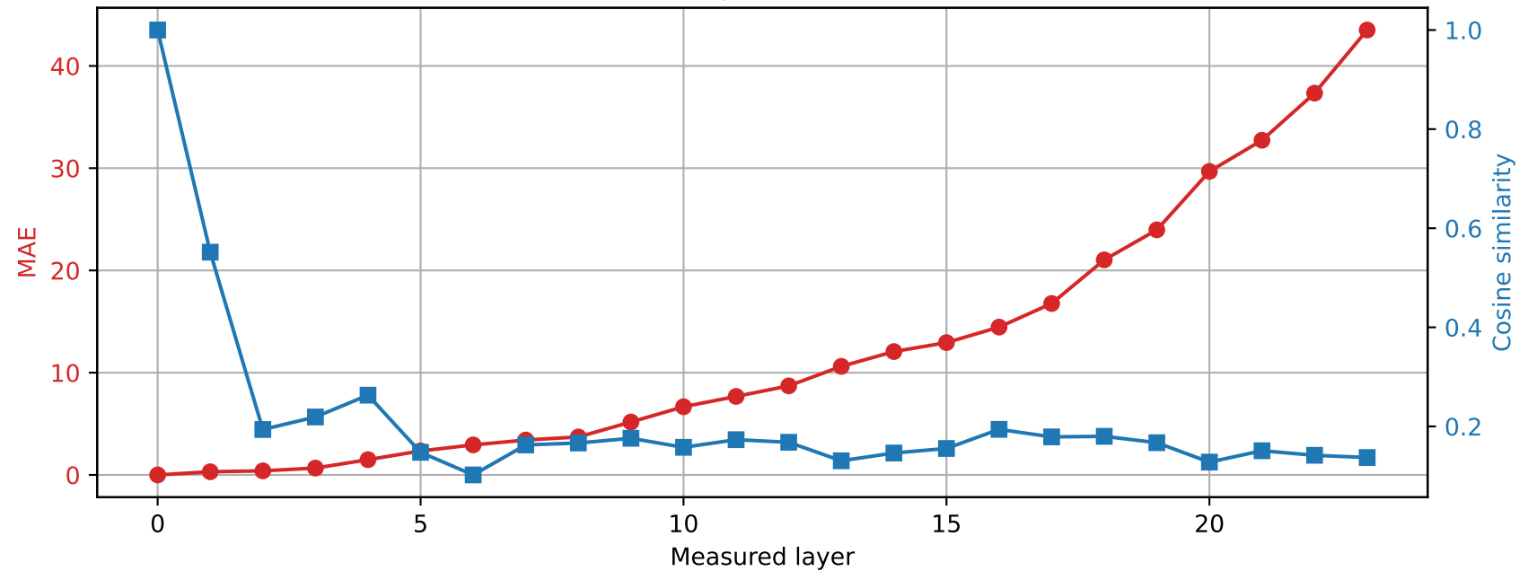
SmolLM2-1.7B-Instruct | Prompt 4 Spared layer 0 | Hybrid vs quantized
