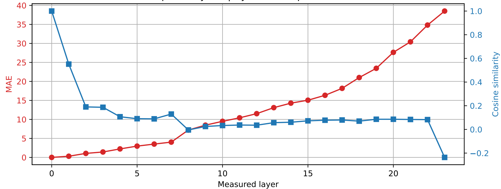
SmolLM2-1.7B-Instruct | Prompt 4 Spared layer 2 | Hybrid vs unquantized
