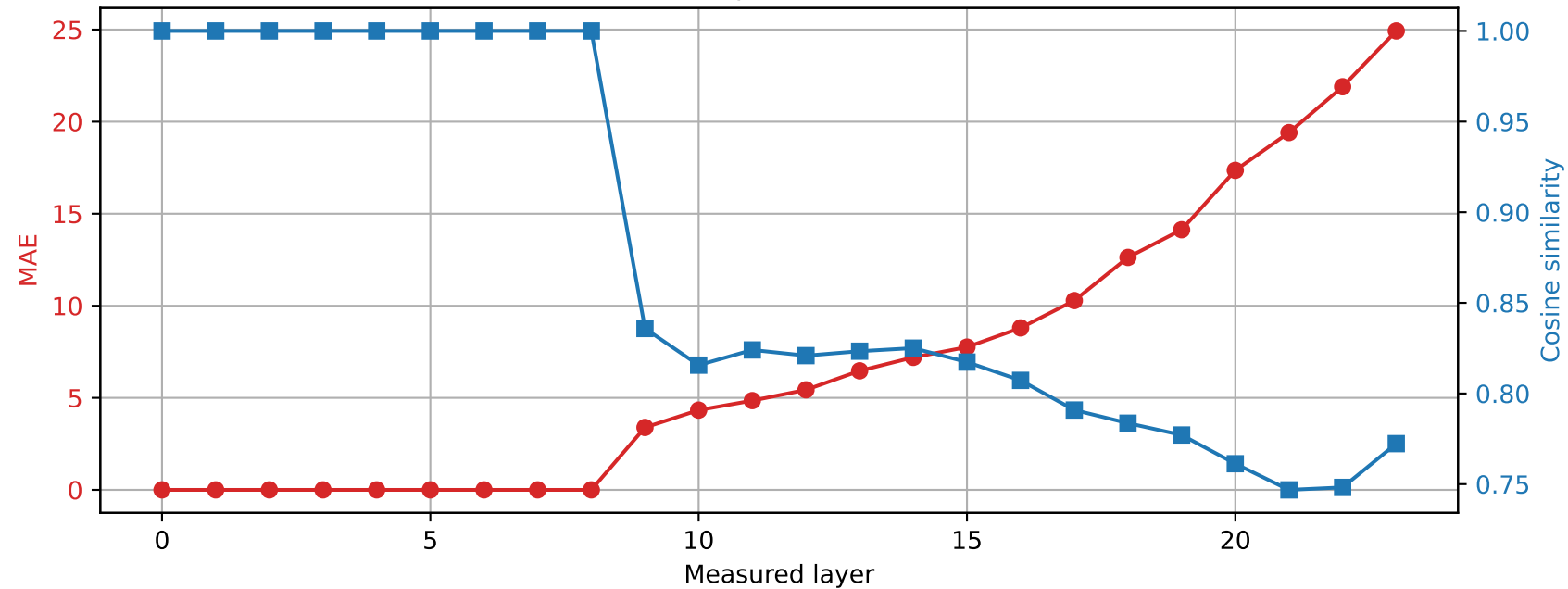
SmolLM2-1.7B-Instruct | Prompt 4 Spared layer 8 | Hybrid vs quantized
