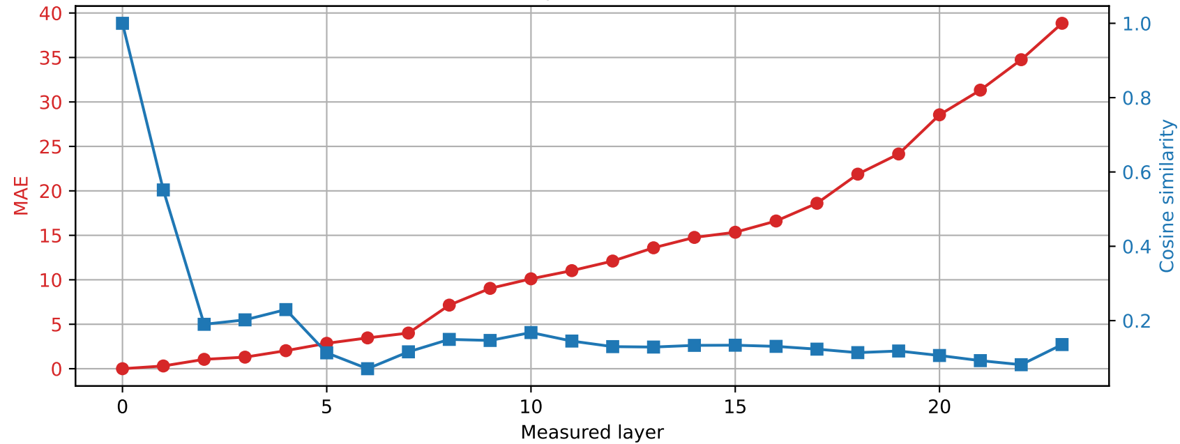
SmolLM2-1.7B-Instruct | Prompt 4 Spared layer 8 | Hybrid vs unquantized
