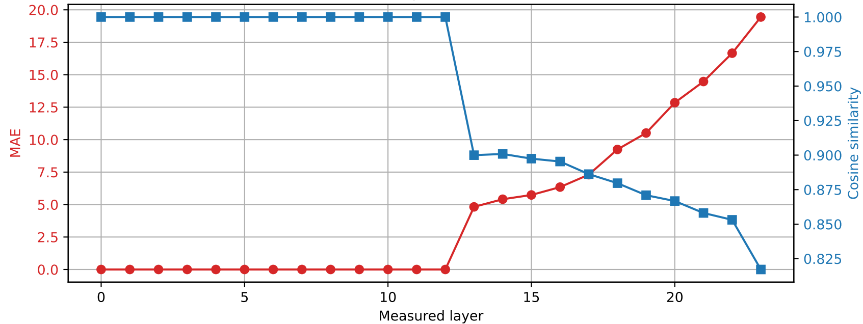
SmolLM2-1.7B-Instruct | Prompt 4 Spared layer 12 | Hybrid vs quantized
