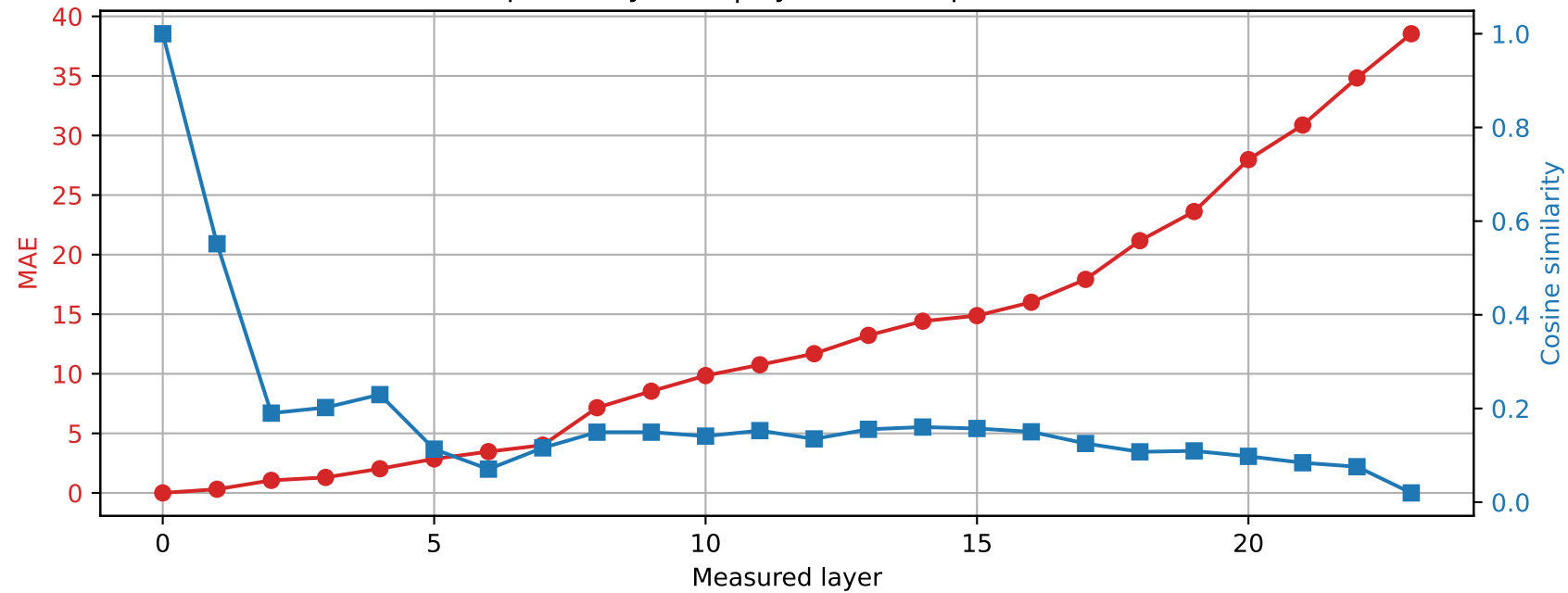
SmolLM2-1.7B-Instruct | Prompt 4 Spared layer 12 | Hybrid vs unquantized
