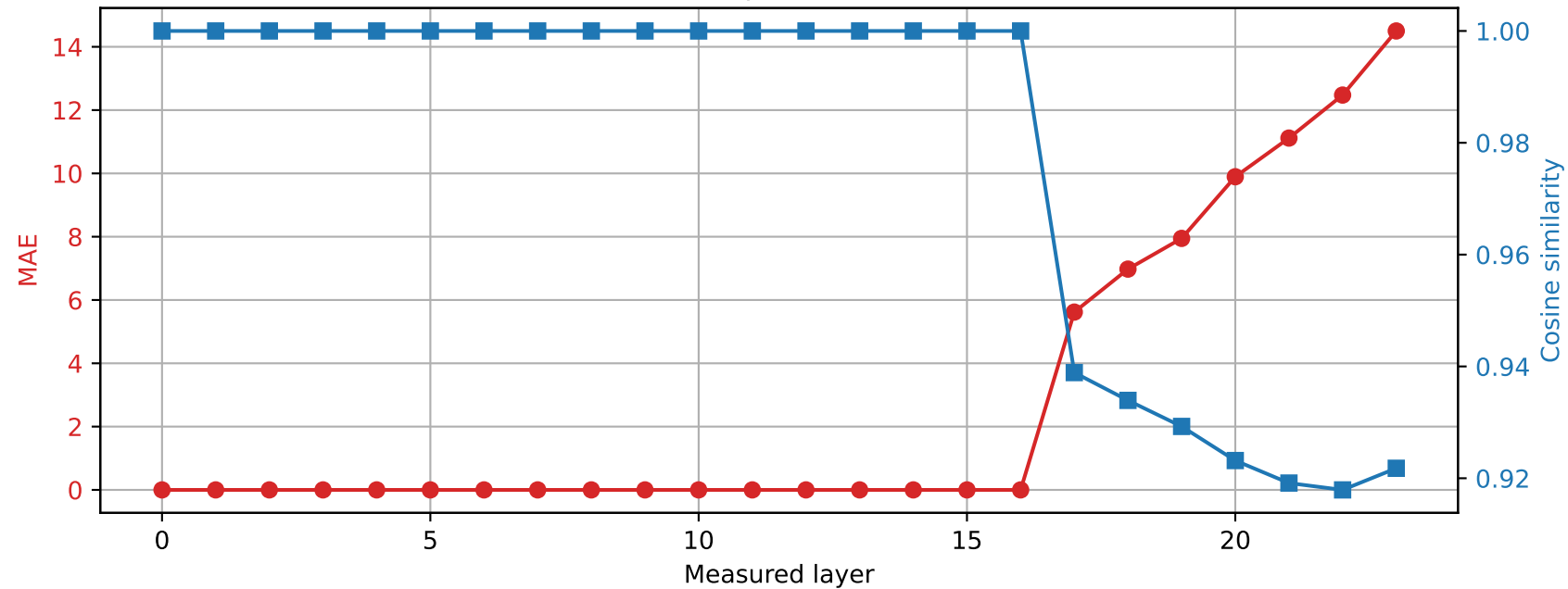
SmolLM2-1.7B-Instruct | Prompt 4 Spared layer 16 | Hybrid vs quantized
