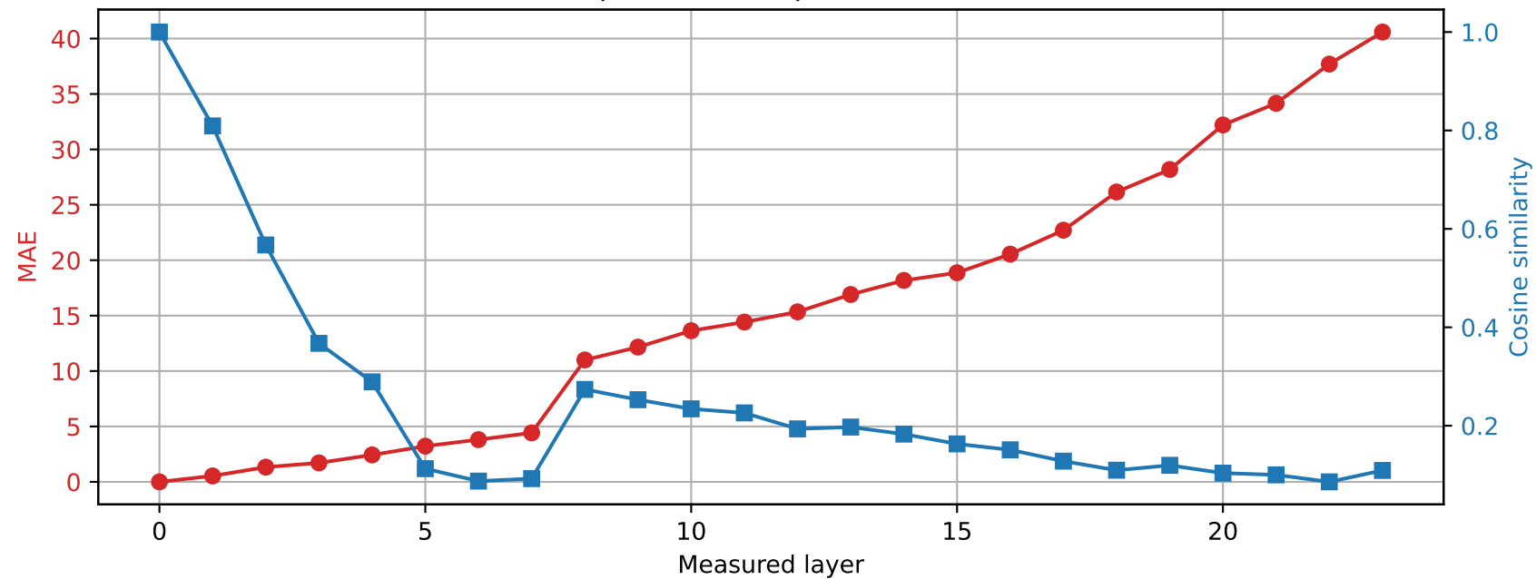
SmolLM2-1.7B-Instruct | Prompt 0 Unquantized vs quantized int4
