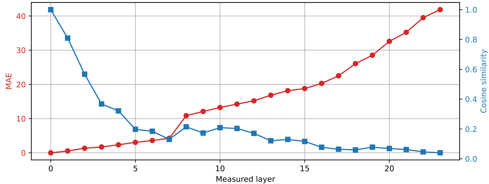
SmolLM2-1.7B-Instruct | Prompt 0 Spared layer 3 | Hybrid vs unquantized
