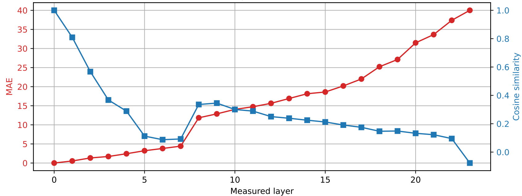
SmolLM2-1.7B-Instruct | Prompt 0 Spared layer 7 | Hybrid vs unquantized
