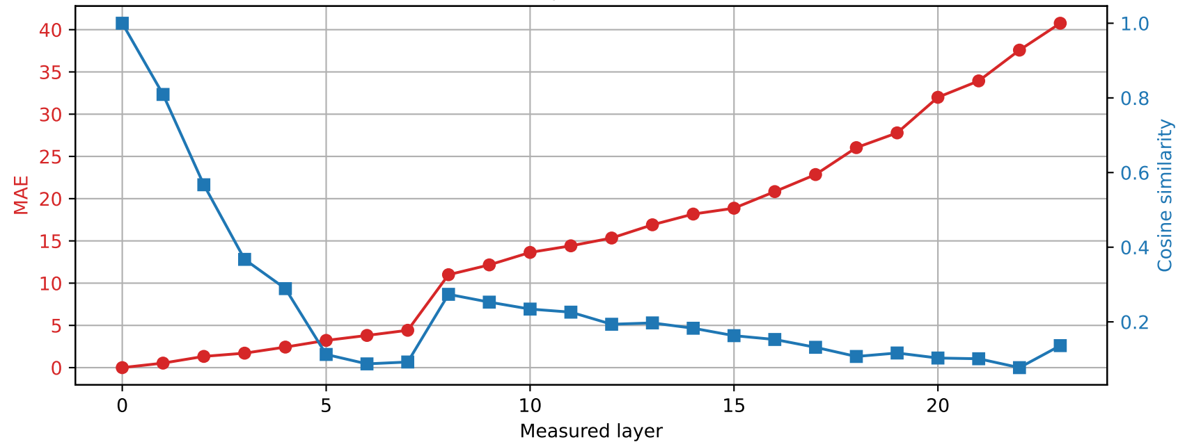
SmolLM2-1.7B-Instruct | Prompt 0 Spared layer 15 | Hybrid vs unquantized
