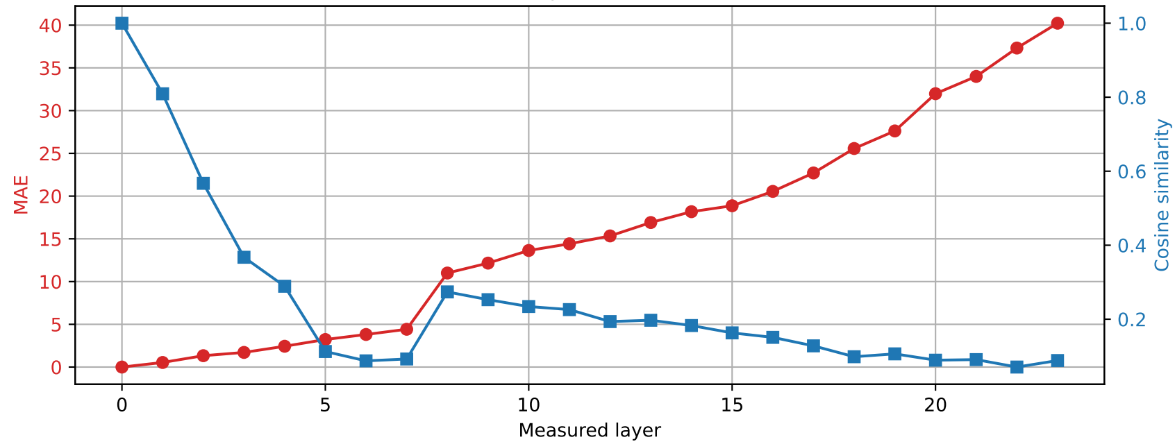
SmolLM2-1.7B-Instruct | Prompt 0 Spared layer 17 | Hybrid vs unquantized
