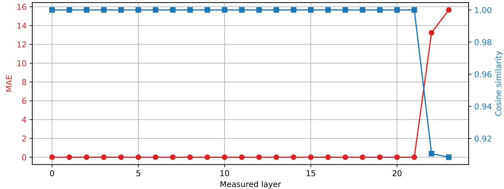
SmolLM2-1.7B-Instruct | Prompt 0 Spared layer 21 | Hybrid vs quantized
