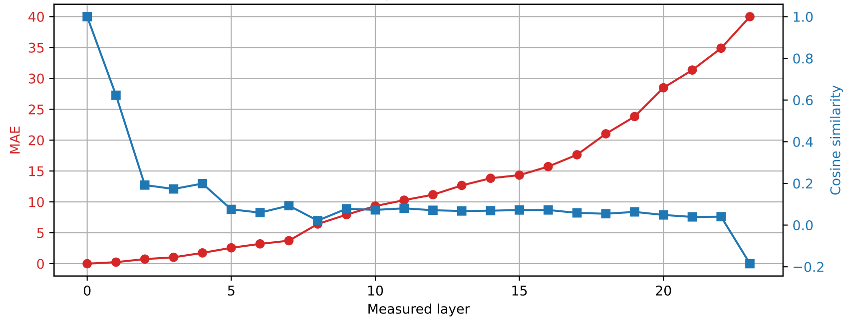
SmolLM2-1.7B-Instruct | Prompt 1 Spared layer 7 | Hybrid vs unquantized
