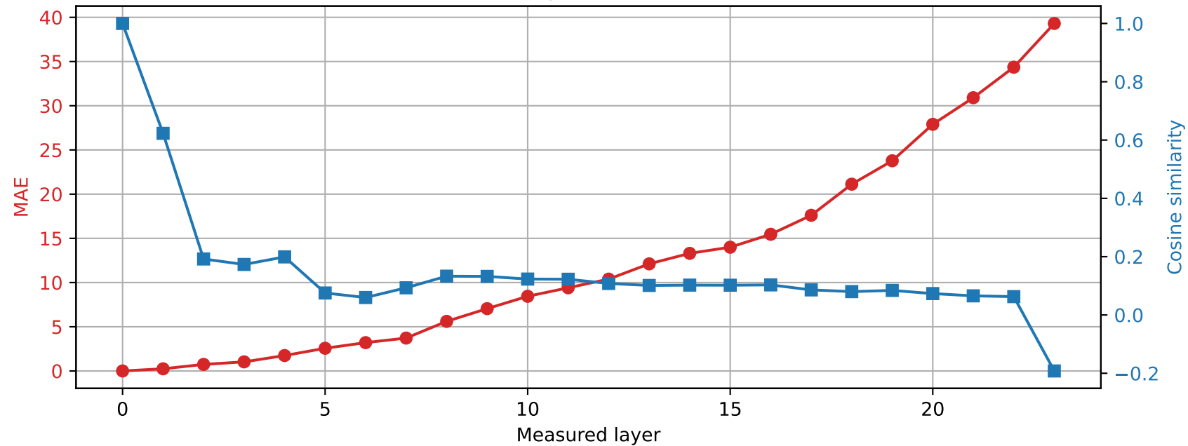
SmolLM2-1.7B-Instruct | Prompt 1 Spared layer 18 | Hybrid vs unquantized
