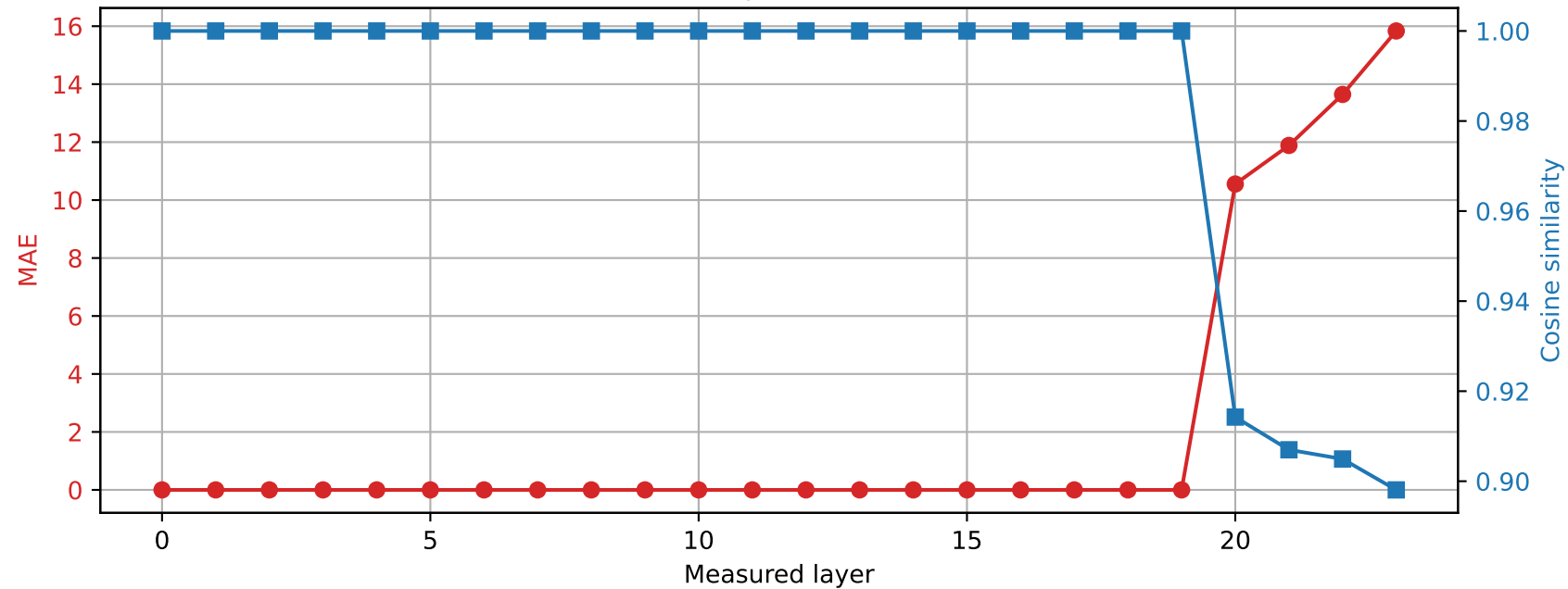
SmolLM2-1.7B-Instruct | Prompt 1 Spared layer 19 | Hybrid vs quantized
