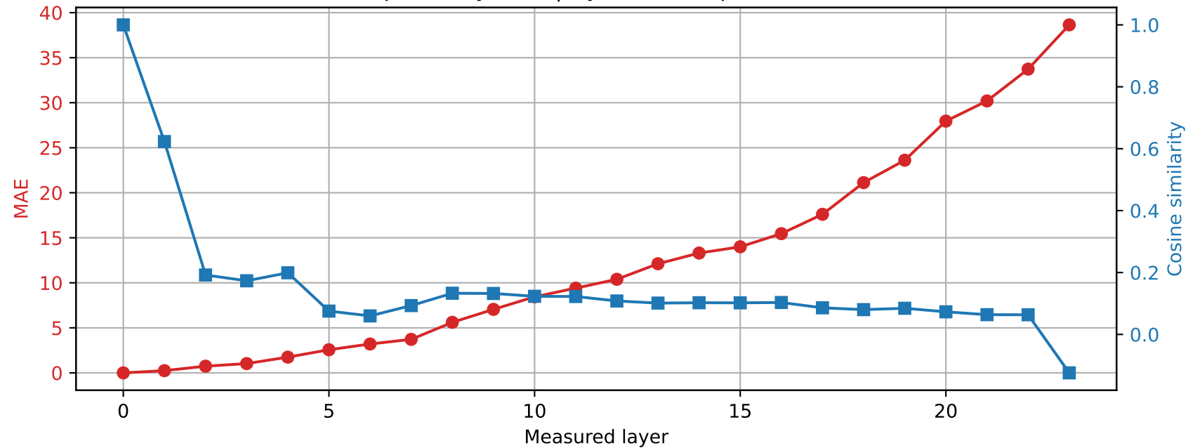
SmolLM2-1.7B-Instruct | Prompt 1 Spared layer 20 | Hybrid vs unquantized
