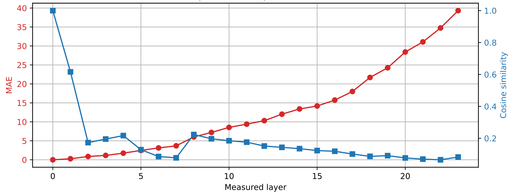
SmolLM2-1.7B-Instruct | Prompt 2 Unquantized vs quantized int4
