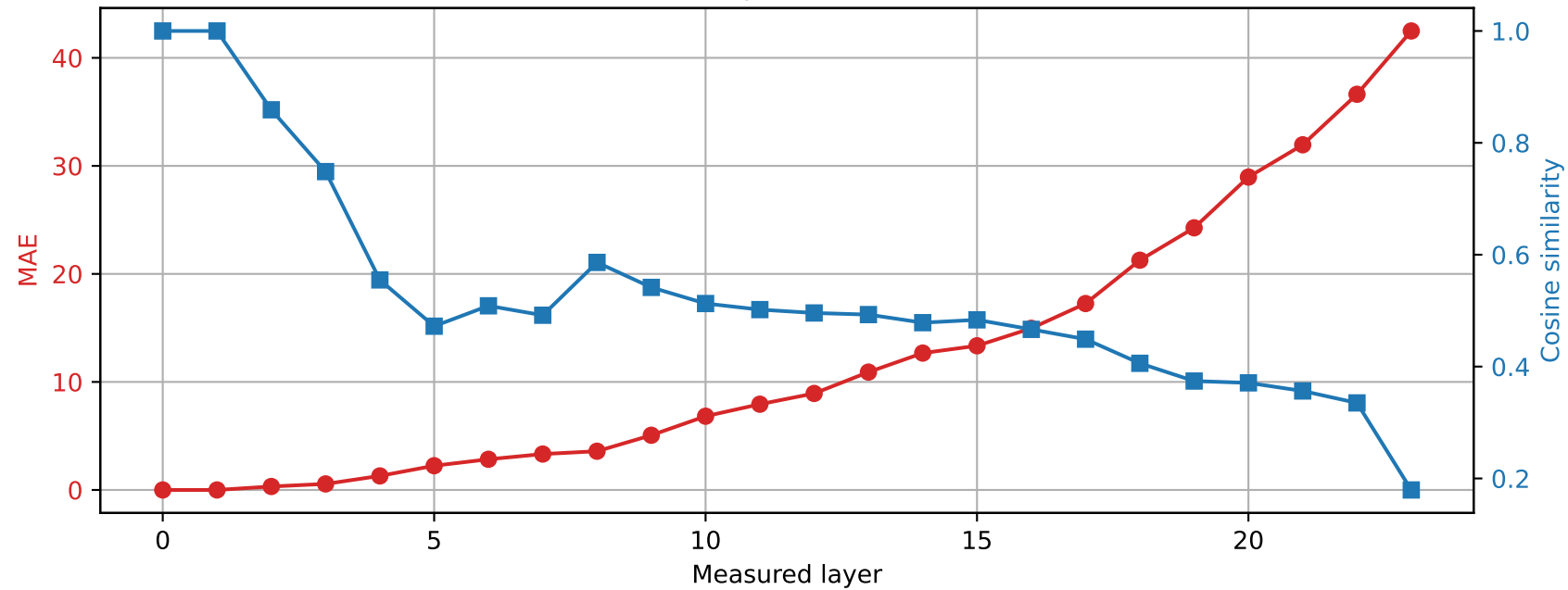
SmolLM2-1.7B-Instruct | Prompt 2 Spared layer 1 | Hybrid vs quantized
