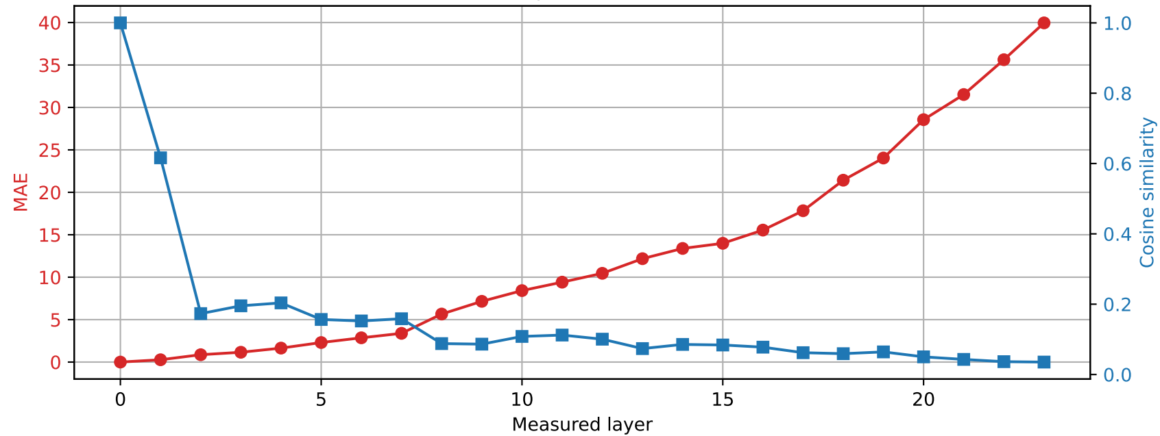
SmolLM2-1.7B-Instruct | Prompt 2 Spared layer 3 | Hybrid vs unquantized
