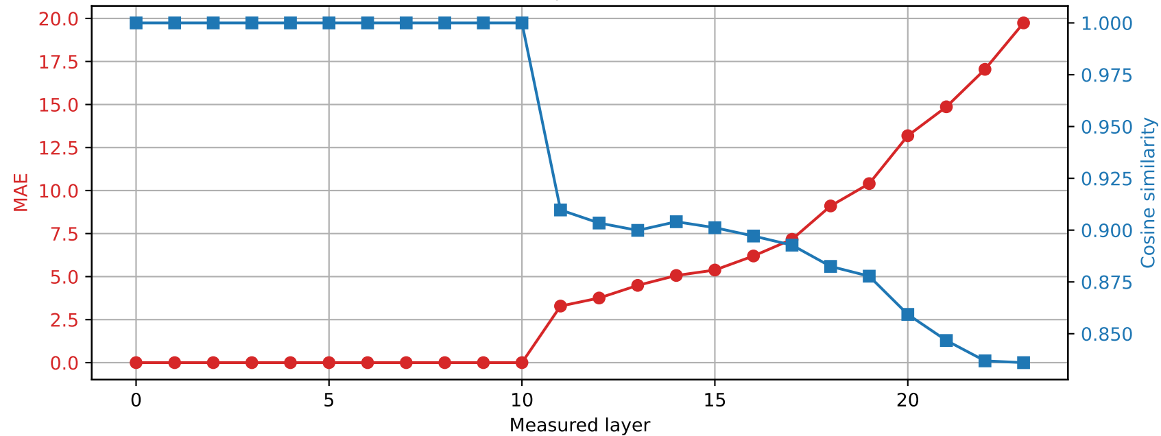
SmolLM2-1.7B-Instruct | Prompt 2 Spared layer 10 | Hybrid vs quantized
