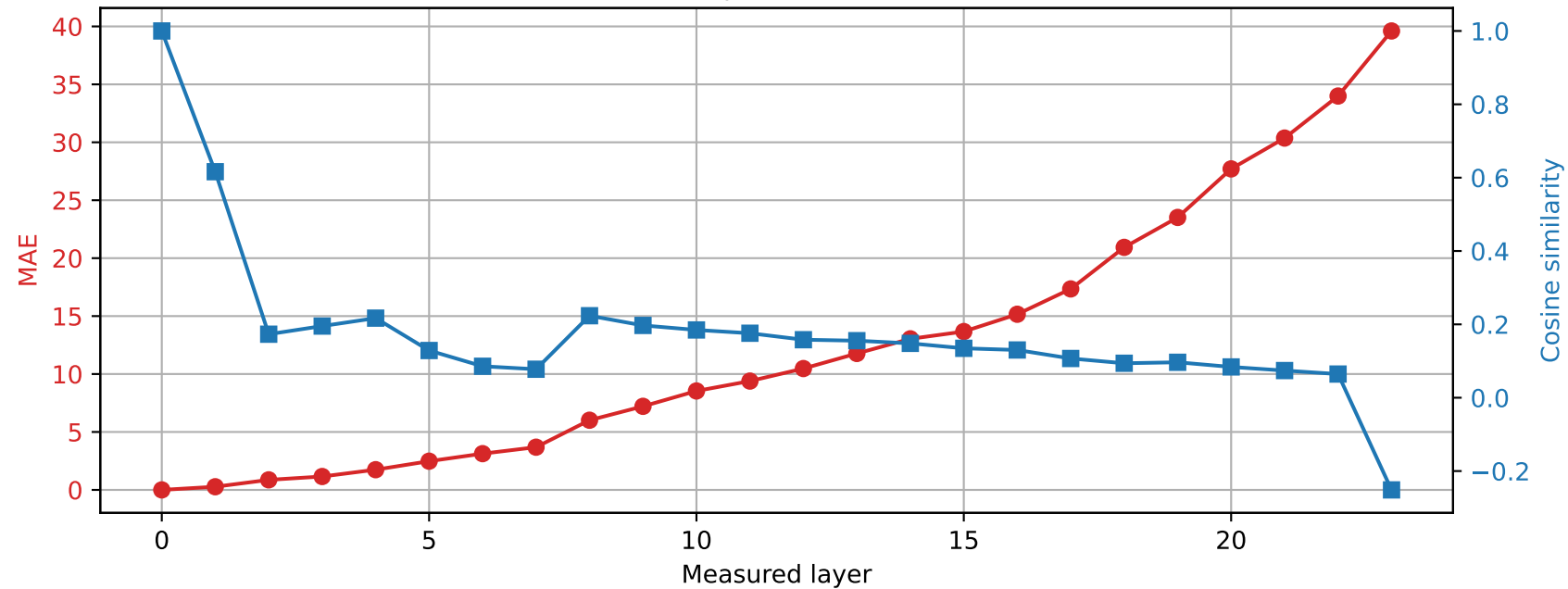
SmolLM2-1.7B-Instruct | Prompt 2 Spared layer 11 | Hybrid vs unquantized
