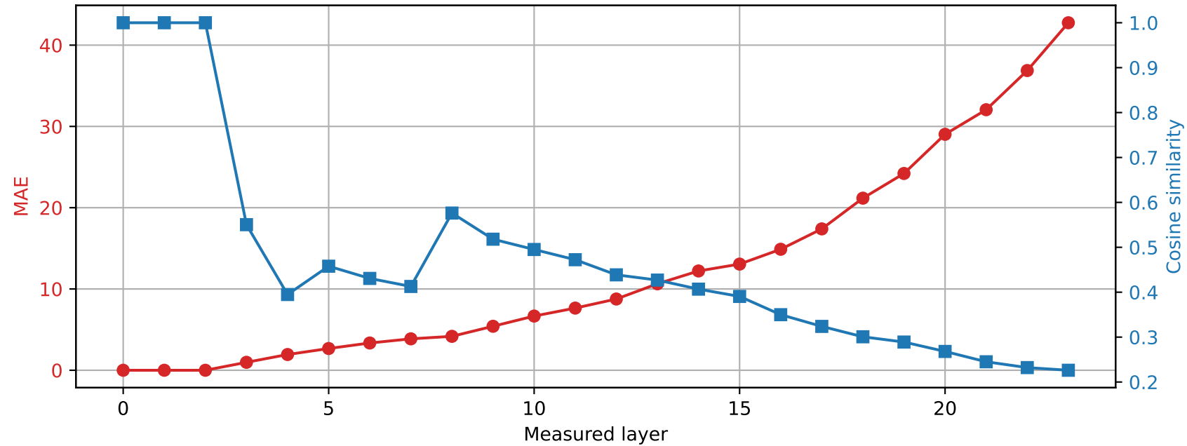
SmolLM2-1.7B-Instruct | Prompt 3 Spared layer 2 | Hybrid vs quantized
