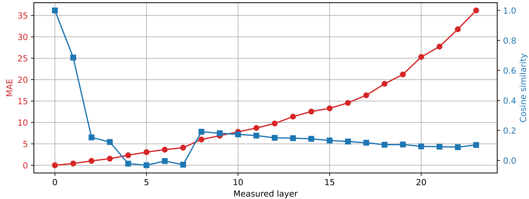
SmolLM2-1.7B-Instruct | Prompt 3 Spared layer 2 | Hybrid vs unquantized
