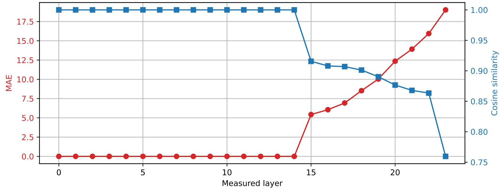
SmolLM2-1.7B-Instruct | Prompt 3 Spared layer 14 | Hybrid vs quantized
