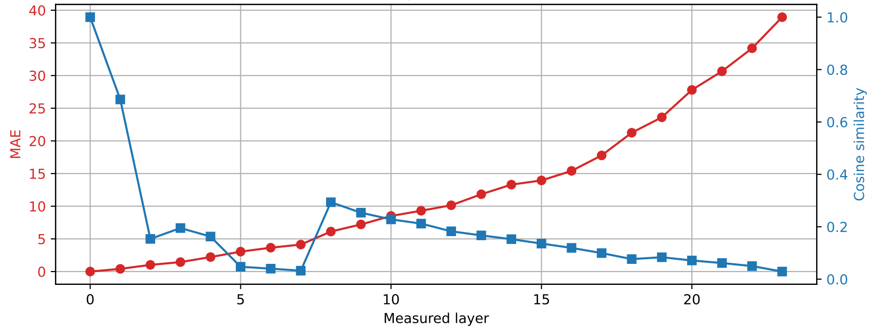
SmolLM2-1.7B-Instruct | Prompt 3 Spared layer 17 | Hybrid vs unquantized
