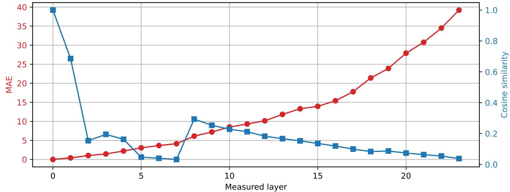
SmolLM2-1.7B-Instruct | Prompt 3 Spared layer 23 | Hybrid vs unquantized
