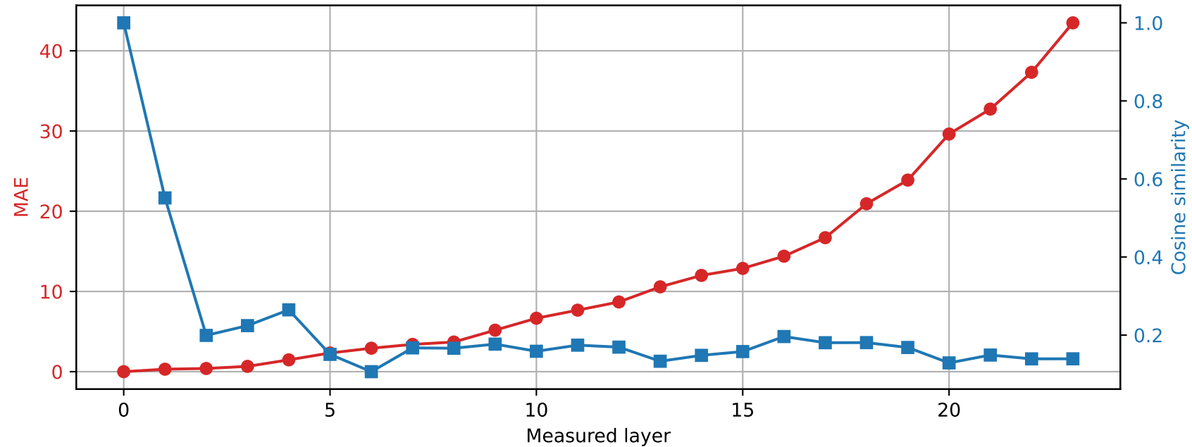
SmolLM2-1.7B-Instruct | Prompt 4 Spared layer 0 | Hybrid vs quantized
