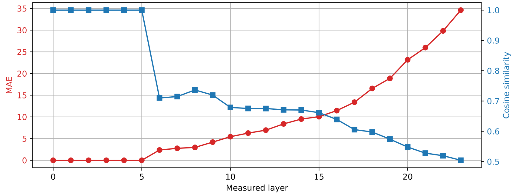
SmolLM2-1.7B-Instruct | Prompt 4 Spared layer 5 | Hybrid vs quantized
