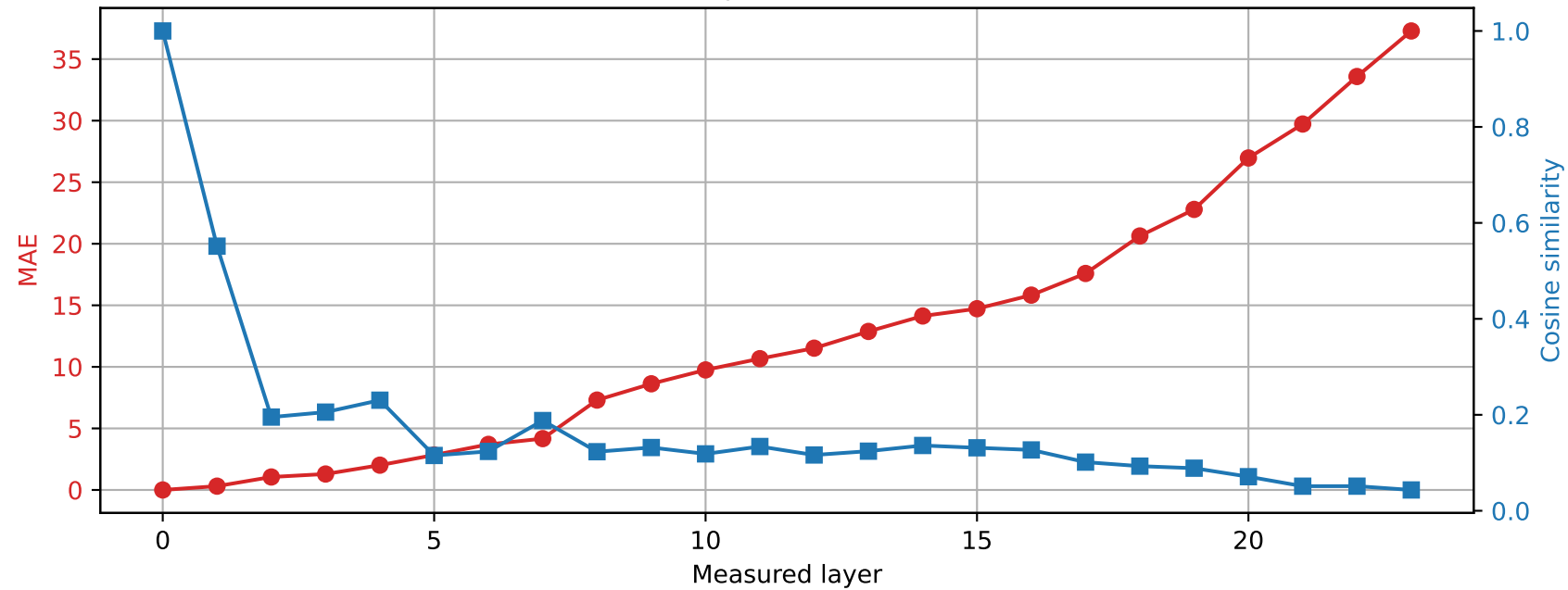
SmolLM2-1.7B-Instruct | Prompt 4 Spared layer 5 | Hybrid vs unquantized
