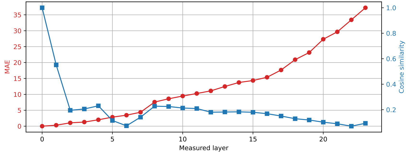
SmolLM2-1.7B-Instruct | Prompt 4 Spared layer 6 | Hybrid vs unquantized
