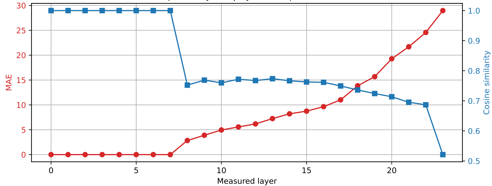
SmolLM2-1.7B-Instruct | Prompt 4 Spared layer 7 | Hybrid vs quantized
