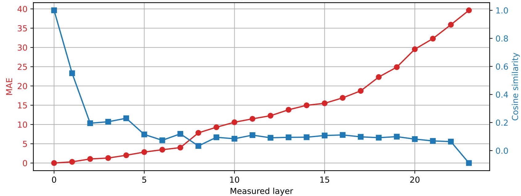
SmolLM2-1.7B-Instruct | Prompt 4 Spared layer 7 | Hybrid vs unquantized
