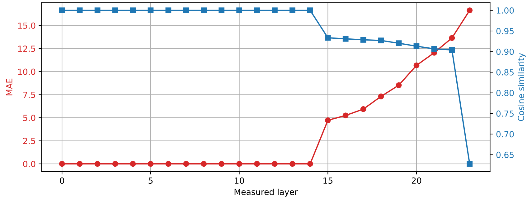
SmolLM2-1.7B-Instruct | Prompt 4 Spared layer 14 | Hybrid vs quantized
