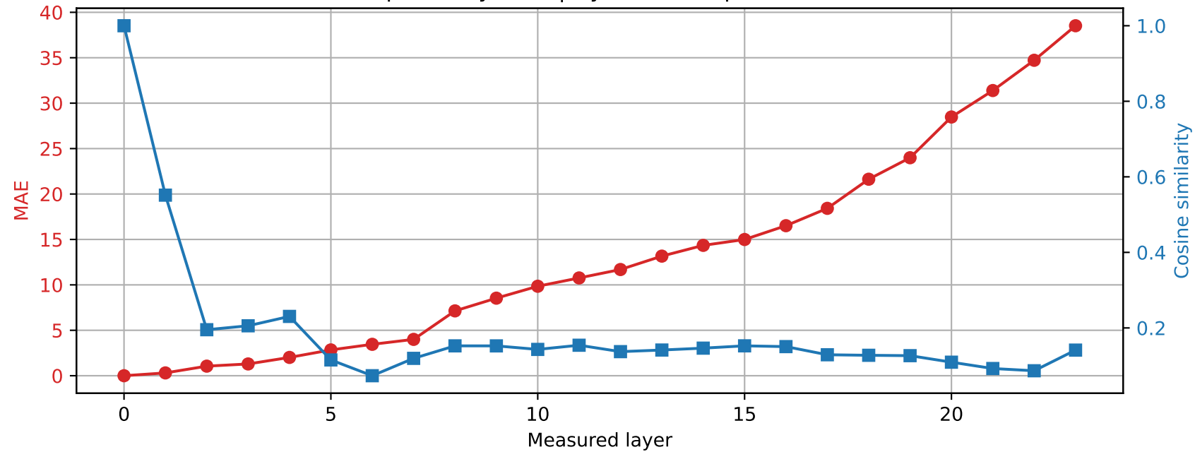
SmolLM2-1.7B-Instruct | Prompt 4 Spared layer 16 | Hybrid vs unquantized
