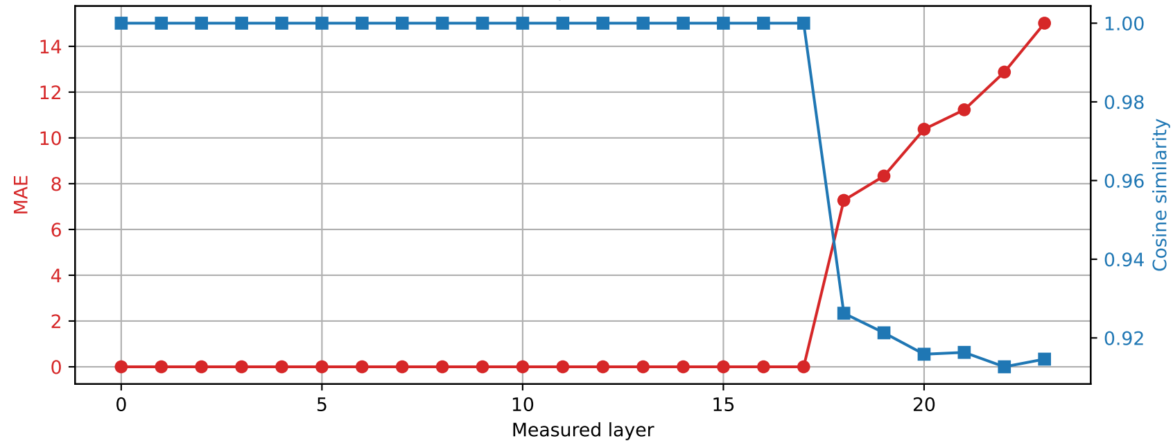
SmolLM2-1.7B-Instruct | Prompt 4 Spared layer 17 | Hybrid vs quantized
