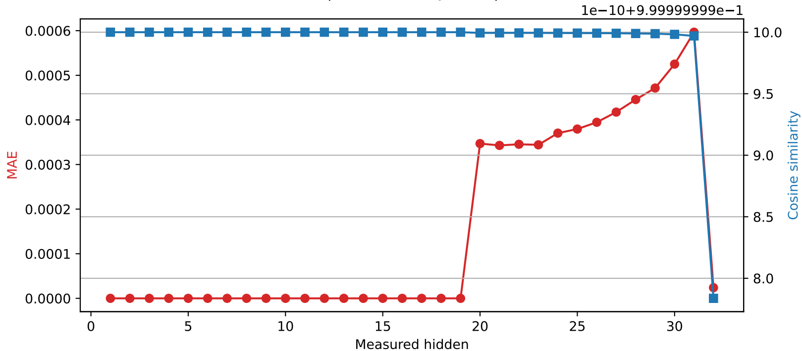
SmolLM2-360M | Quantized layer 19 | float32 → int16
