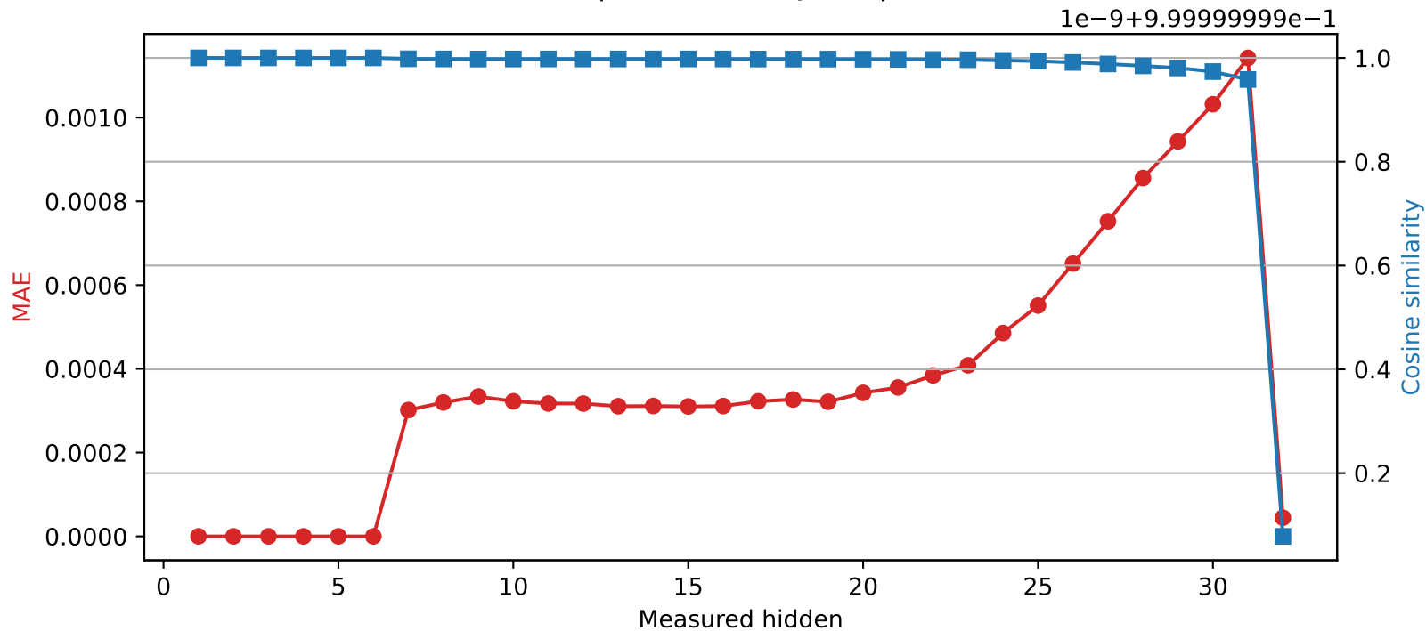
SmolLM2-360M | Quantized layer 6 | float32 → int16
