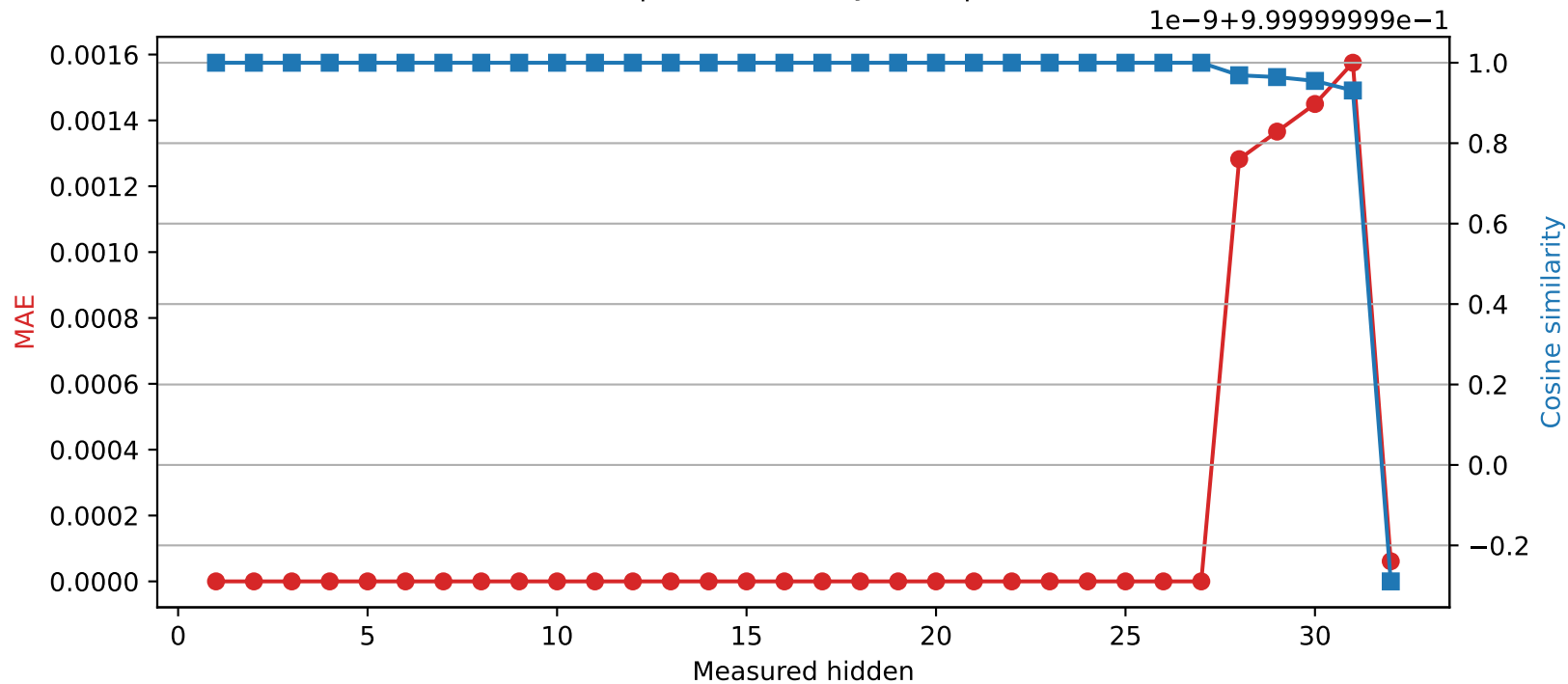
SmolLM2-360M | Quantized layer 27 | float32 → int16
