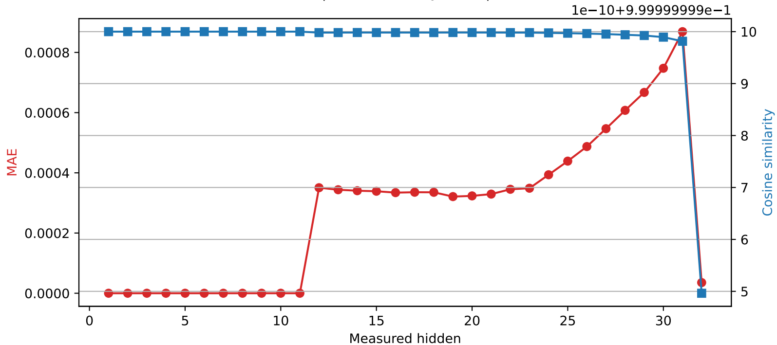
SmolLM2-360M | Quantized layer 11 | float32 → int16
