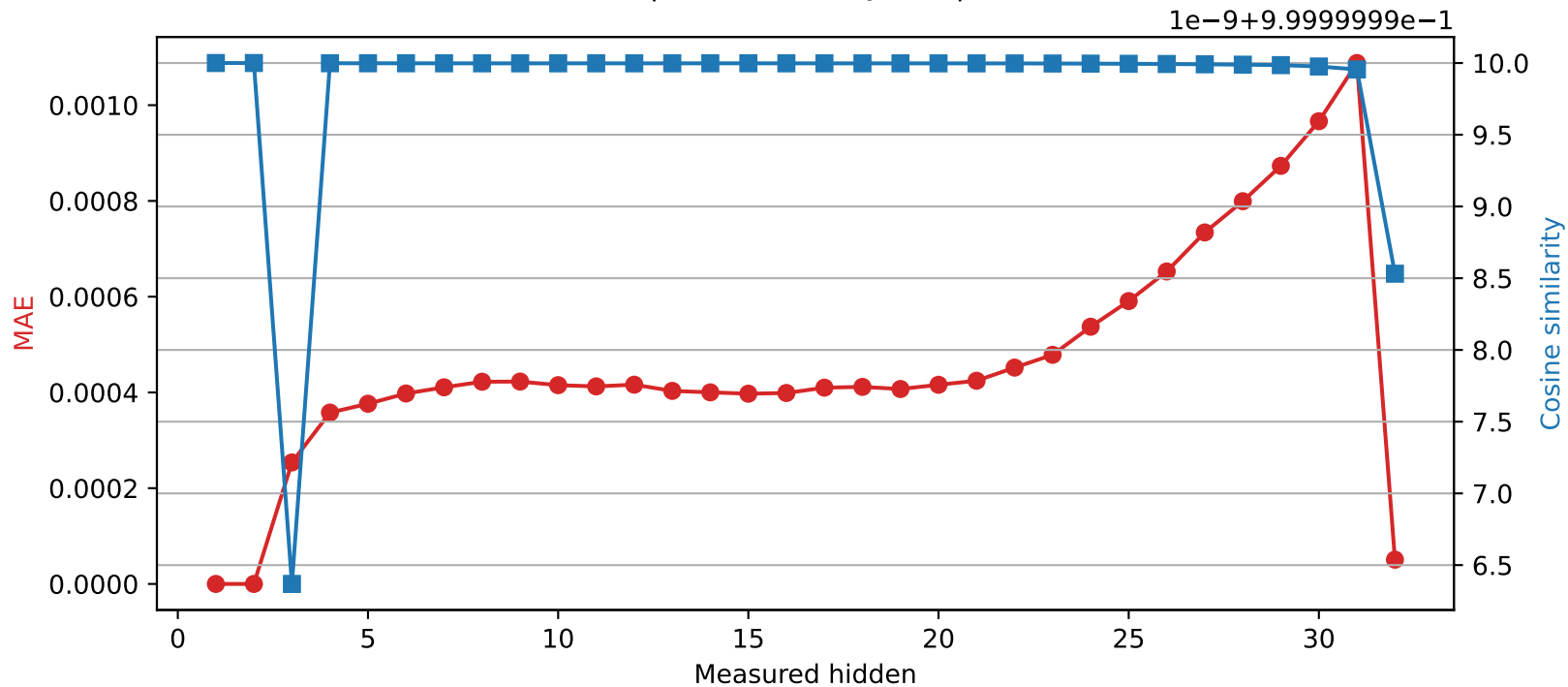
SmolLM2-360M | Quantized layer 2 | float32 → int16
