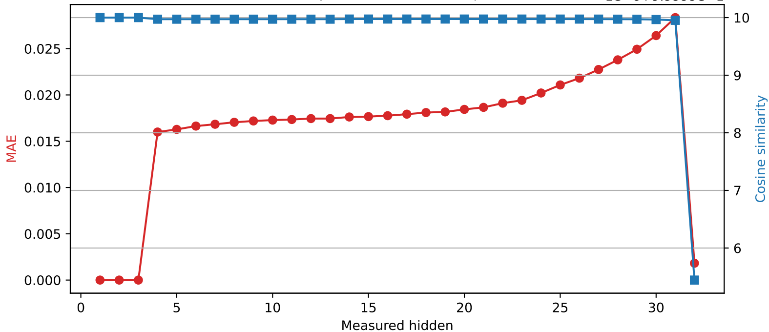
SmolLM2-360M | Quantized layer 3 | float32 \rightarrow int16 1e-6+9.9999e-1
