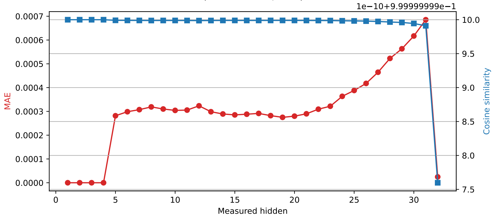
SmolLM2-360M | Quantized layer 4 | float32 → int16
