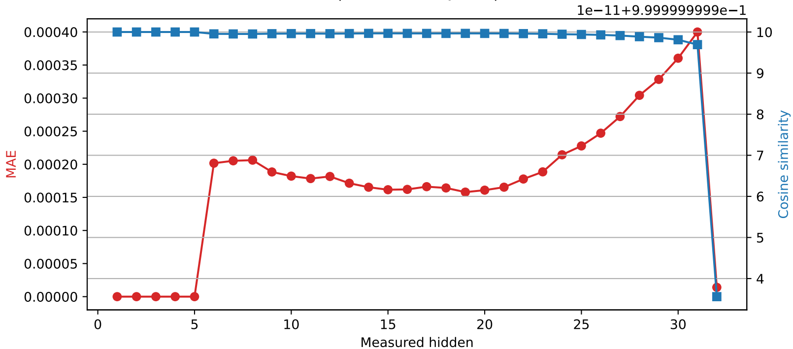
SmolLM2-360M | Quantized layer 5 | float32 → int16
