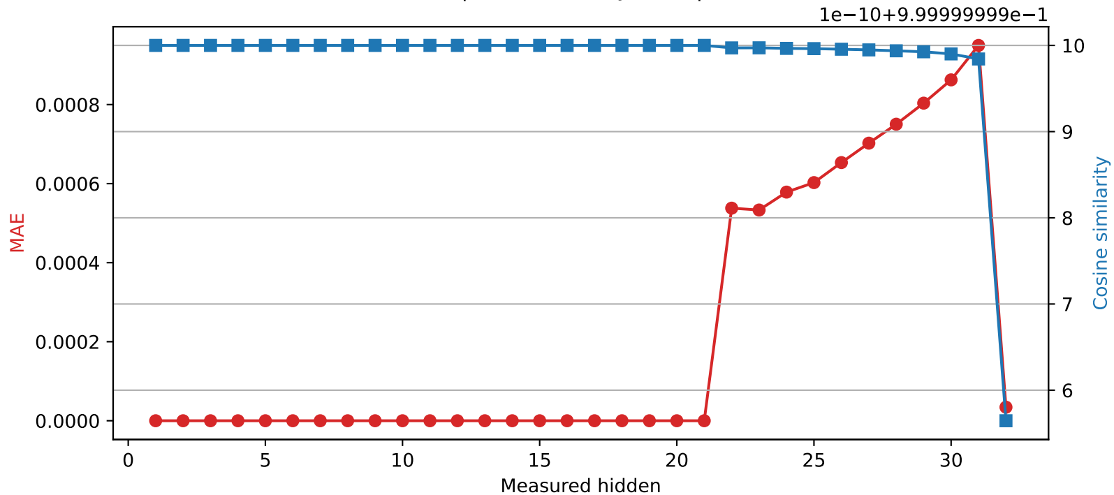
SmolLM2-360M | Quantized layer 21 | float32 \rightarrow int16
