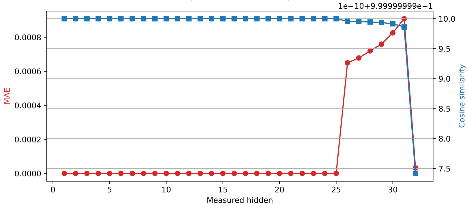
SmolLM2-360M | Quantized layer 25 | float32 → int16
