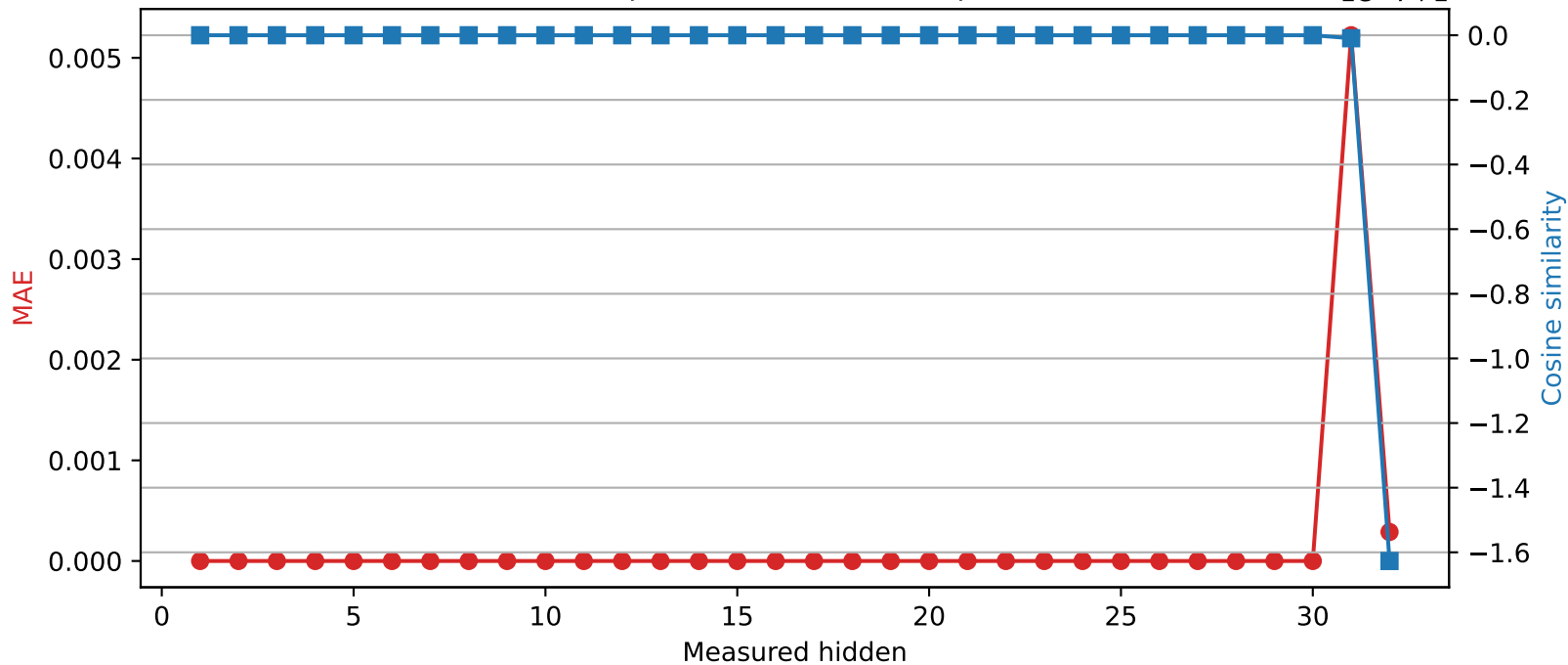
SmolLM2-360M | Quantized layer 30 | float32 → int16
