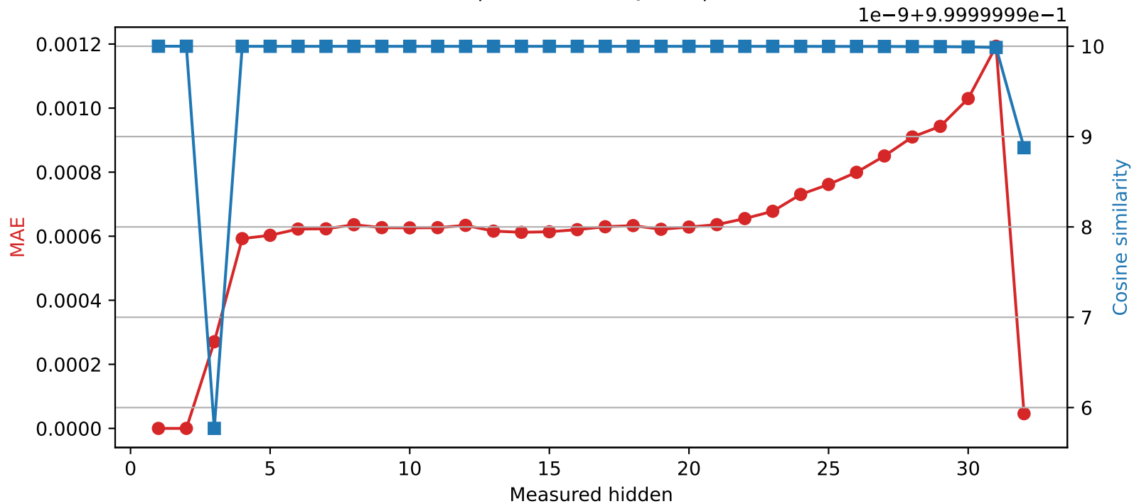
SmolLM2-360M | Quantized layer 2 | float64 → int16
