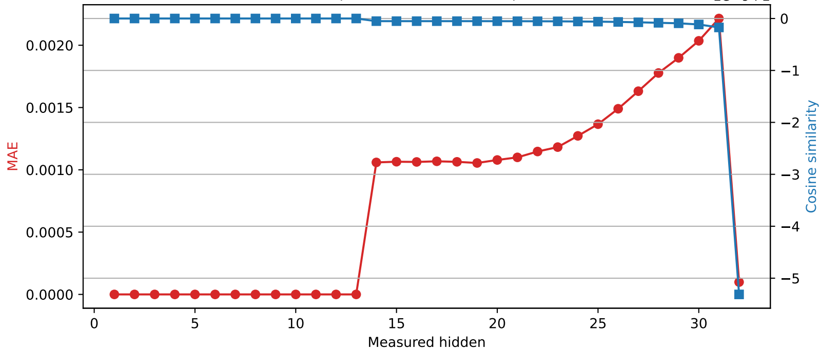
SmolLM2-360M | Quantized layer 13 | float64 → int16
