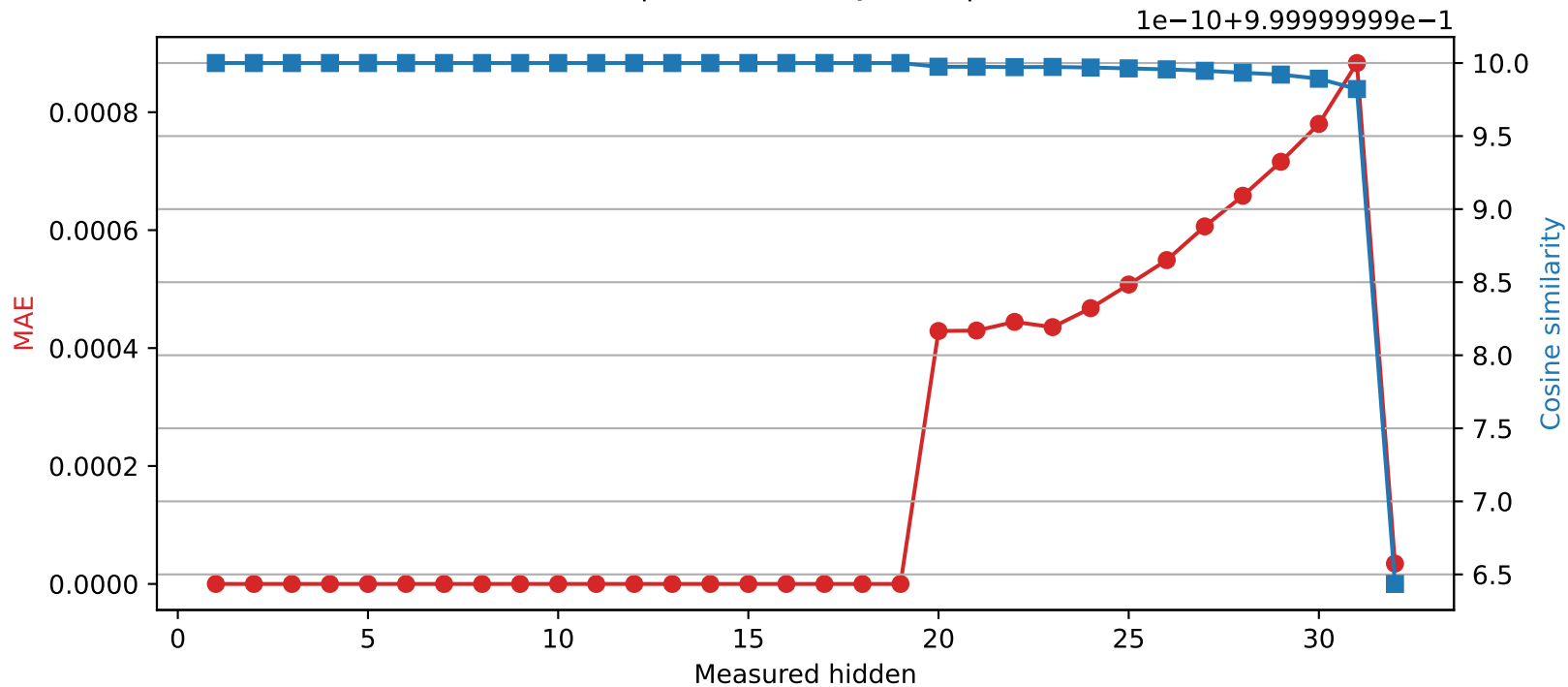
SmolLM2-360M | Quantized layer 19 | float64 → int16
